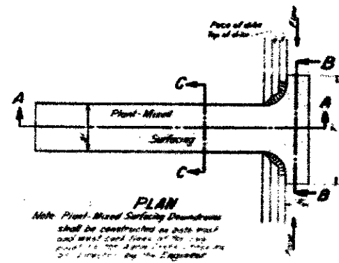
PLANT-MIXED SURFACING SPILLWAY DOWNDRAIN Scale: 1"=4'
